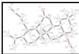
Fig. 1. The molecular structure of (I) showing the atomic labelling scheme. Non-H atoms are drawn as 30% probability displacement ellipsoids; H atoms are shown as small spheres of arbitrary radius.
